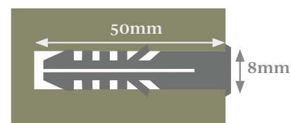
8 x 50mm Drilling Diagram
