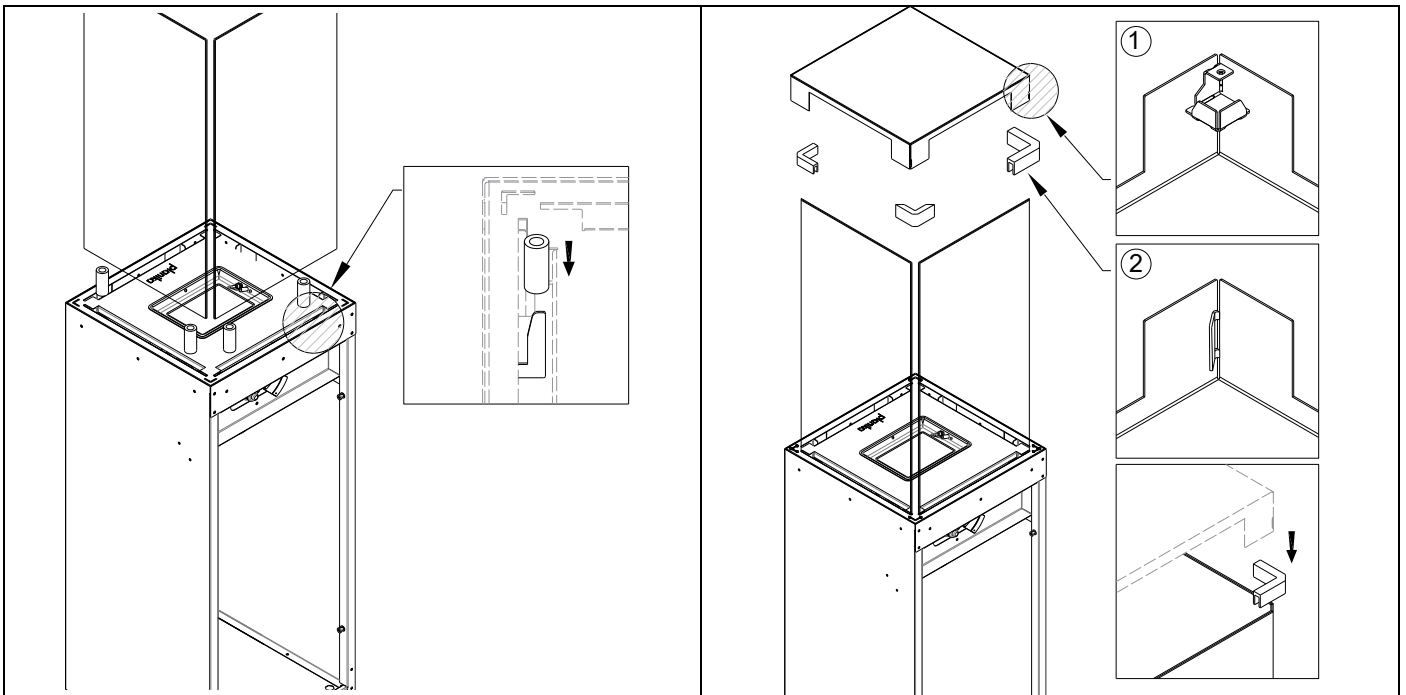
Fig 5– Installation of the glass in slots and metal hood on glass
